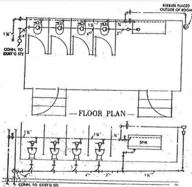
— ELEVATION — TYPICAL TEMPORARY TOILET ROOM
